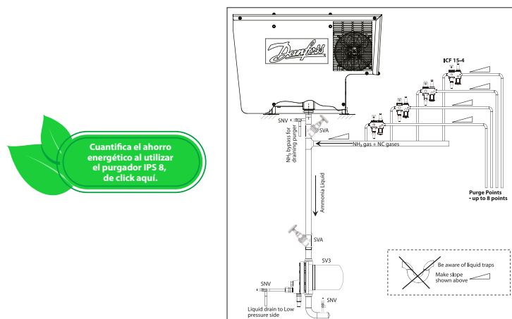
Fig. 10 Multi-point purging from up to 8 purging points
